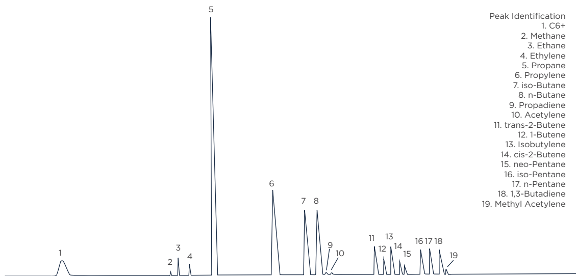
Figure 1, Chromatogram for ASTM D2163.
