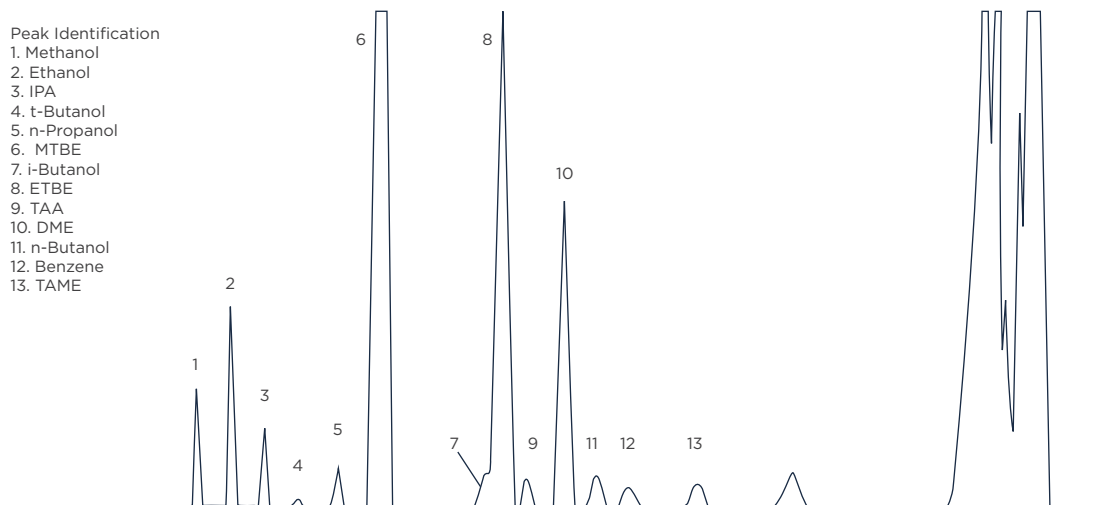
Figure 1, Chromatogram for ASTM D4815
